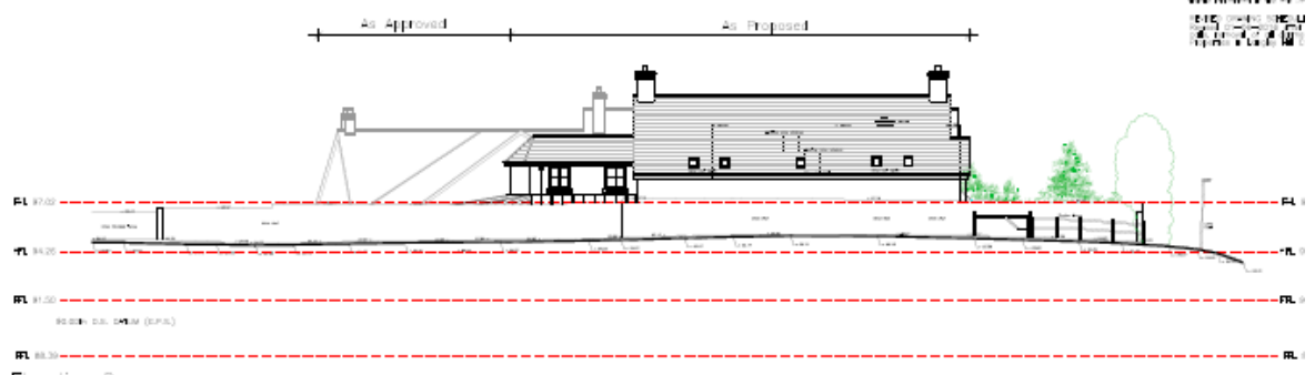
Elevation 2 Street Scene As Proposed Lingley Hill Close
