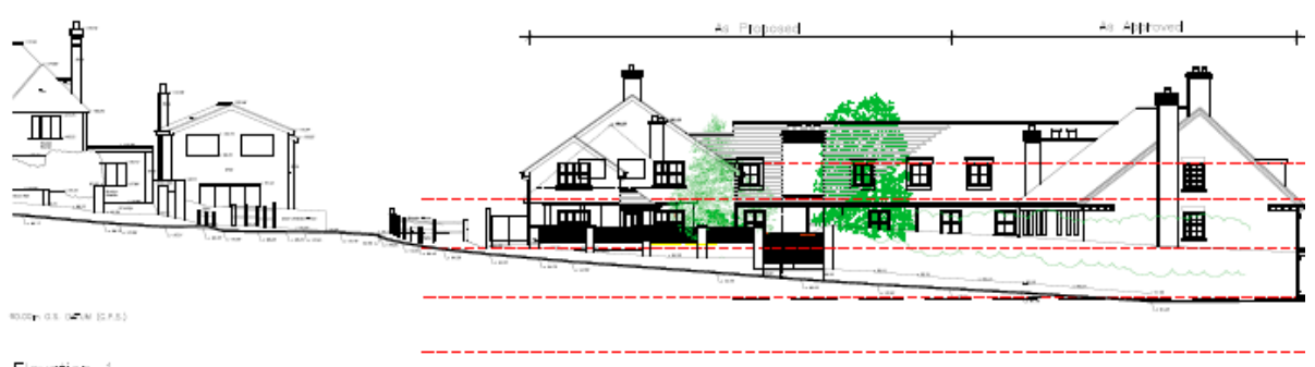
Elevation 1 Street Scene As Proposed Lingley Hill
